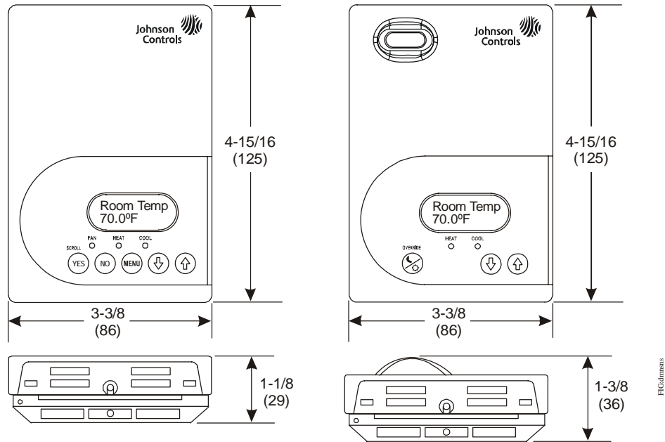
Figure 5: TEC2664Z-2 Rooftop Controller (Left) and TEC2647Z-2+PIR Zone Controller (Right) Dimensions, in. (mm)
