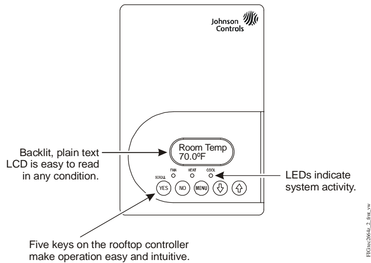
Figure 4: Front Cover of TEC2664Z-2 Rooftop Controller
