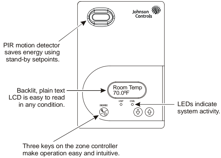
Figure 3: Front Cover of TEC2647Z-2+PIR Zone Controller
