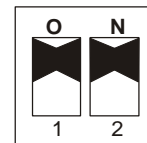
Figure 9: FC Bus EOL Switches in the Initial Factory ON Position
