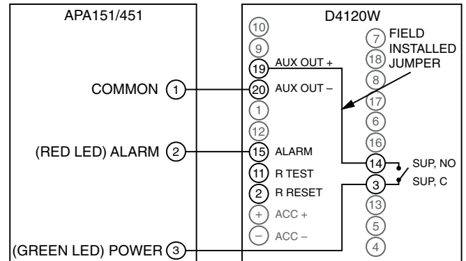
FIGURE 12. WIRING DIAGRAM FOR D4120W TO APA151 OR APA451:
