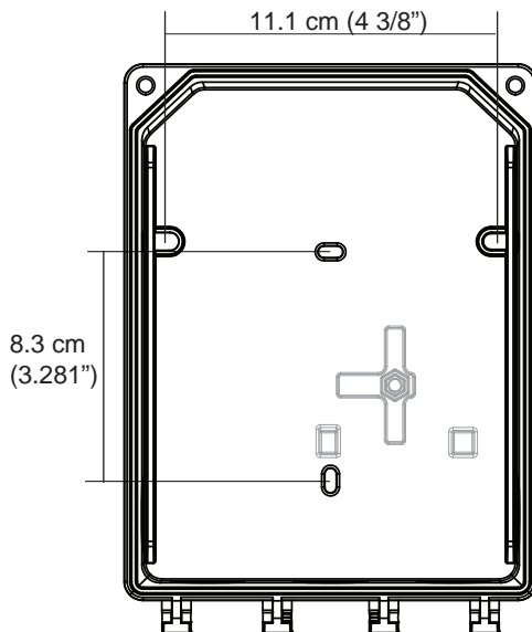
Figure 1. Unit Dimensions
